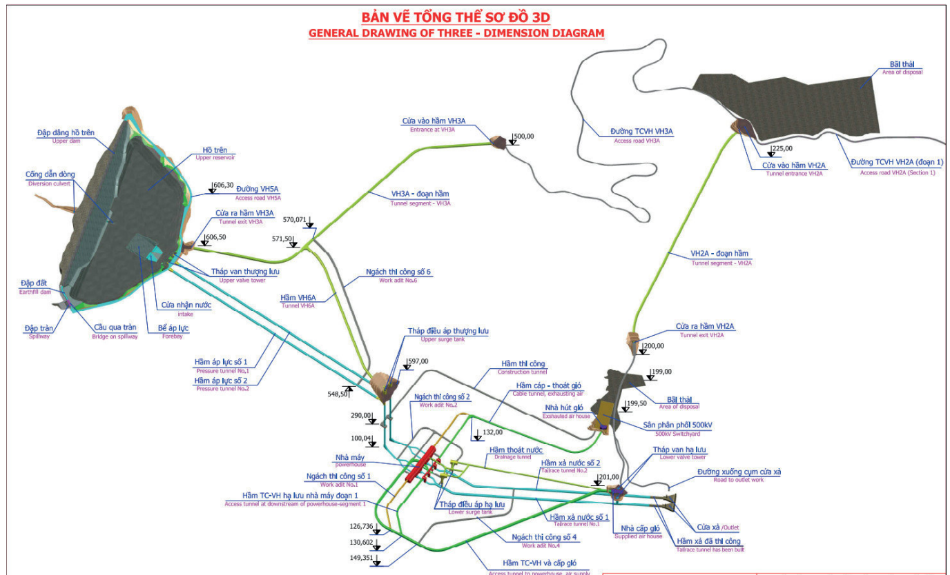
General Drawing of 3D Diagram
